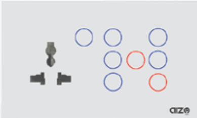
7A 7 Gang with 16A Socket Model Number: LS7-SK1-WC-RSWF Size: 145mm*86mm*34mm
