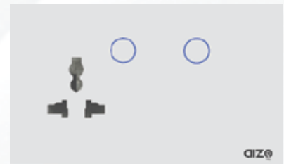
16A 1 Gang with 16A Socket Model Number: HS1-SK1-WC-RSWF Size: 145mm*86mm*34mm
