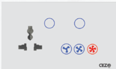
1 Gang 7A Switch, Fan Regulator with 16A Socket Model Number: LS1-FR-SK1-WC-RSWF Size: 145mm*86mm*34mm
